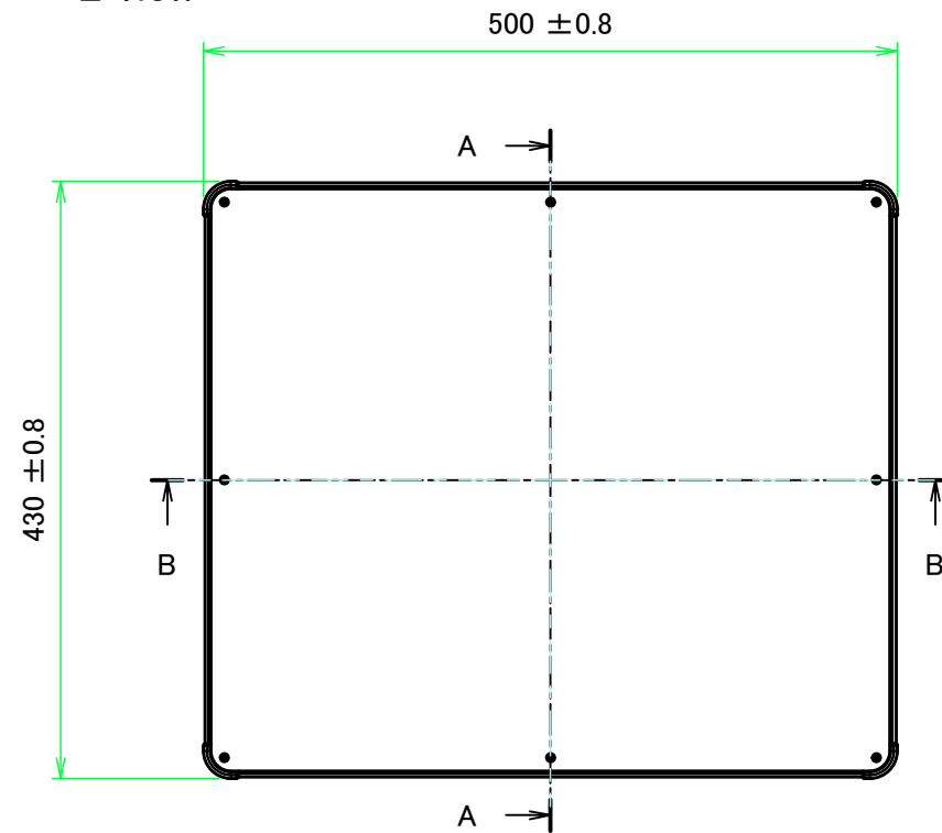
E view
